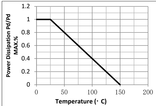
Fig.3 Power Dissipation
